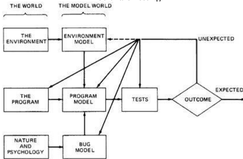
Figure 1.1: A Model for Testing
